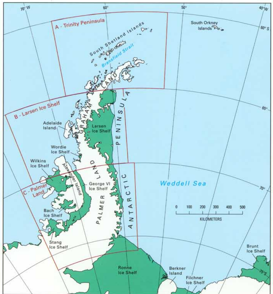
Figure 2. Locations and names of three Antarctic Peninsula areas for which the U.S. Geological Survey and the British Antarctic Survey are preparing coastal-change and glaciological maps (I-2600-A, B, and C, scale 1:1,000,000).
