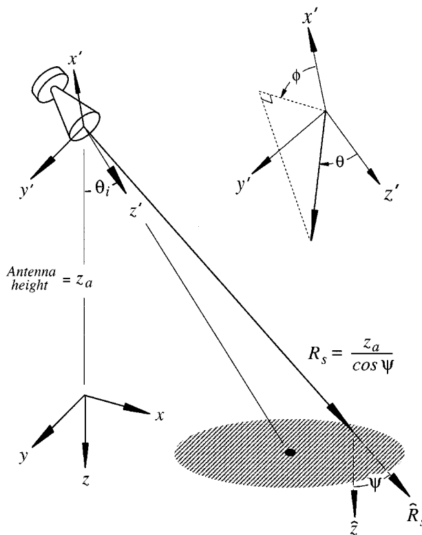
Fig. 1. Antenna at height z_a illuminating the surface z = 0 , with the shaded region corresponding to the main antenna beam.
