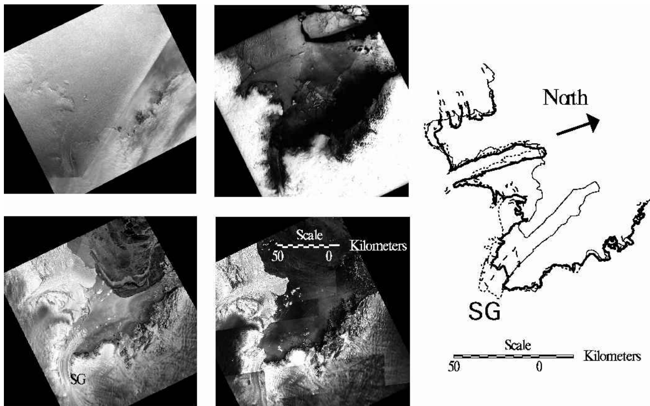
Fig. 5. Shirase Glacier imaged by the Argon satellite in 1963 (upper left), Landsat in 1988 (upper center), RADARSAT-1 in 1997 (lower left) and RADARSAT-1 in 2000 (lower center). Images are centered at 69^{\circ}40' S , 38^{\circ}50' E . The Shirase Glacier (SG) line map on the right depicts the 1963 coastline (thin solid line), the 1988 coastline (short dashed line), the 1997 coastline (long dashed line) and the 2000 coastline (heavy solid line).
