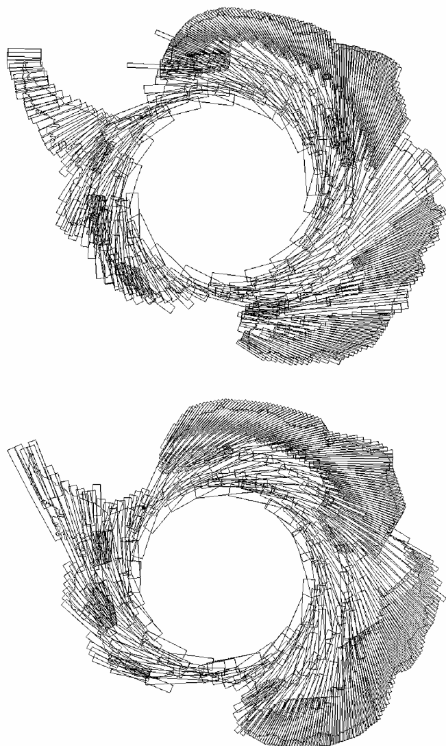
Fig. 1. Ascending (upper) and descending (lower) cumulative-coverage maps for the three MAMM acquisition cycles. Maximum southerly coverage is 80.1^\circ S.
