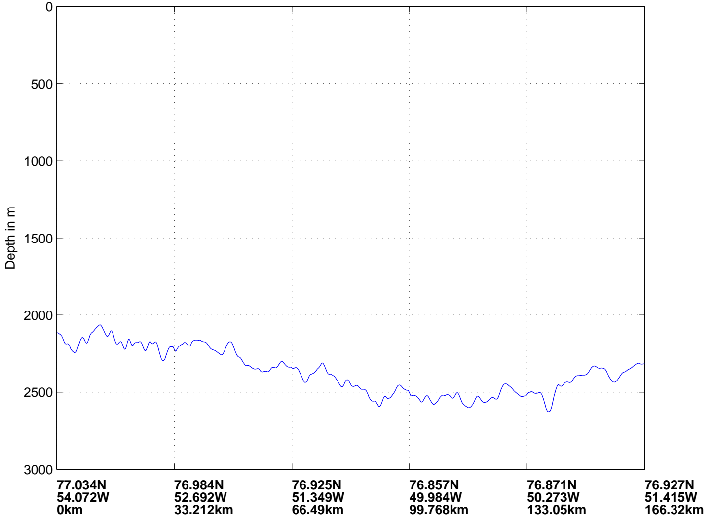
Thickness plot along flightline, section2files(25-49) 23May06
