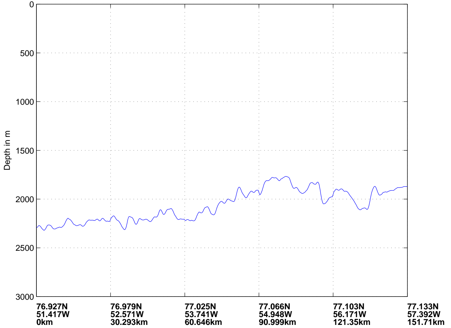
Thickness plot along flightline, section3files(50-74) 23May06
