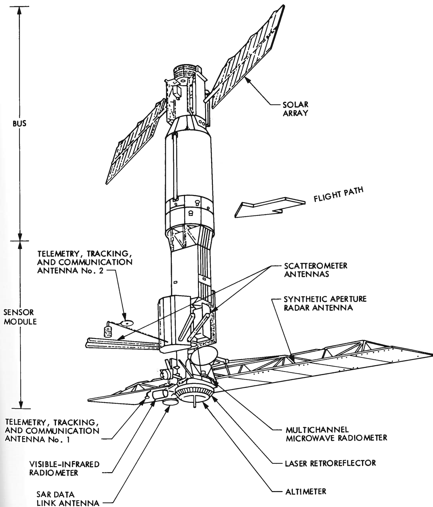
Figure A-1. Seasat bus and payload configuration
