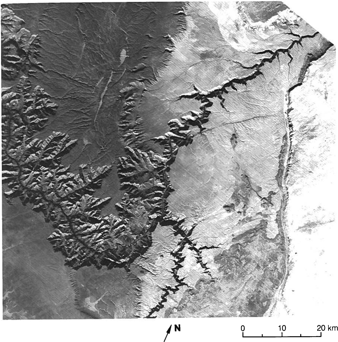
displacement faults associated with the Kaibab upwarp. The doubled features (F2) result from a change in the radar settings. (Seasat image from Rev. 322; Landsat scene ID: 1464-17354.)
